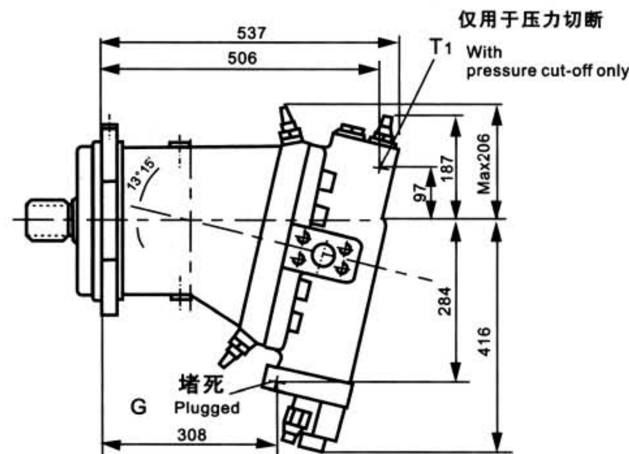
HD液控变量 Hydraulic Control, Pressure Related
