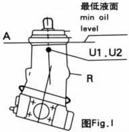
图Fig.1 Mounting on Top of Tank
