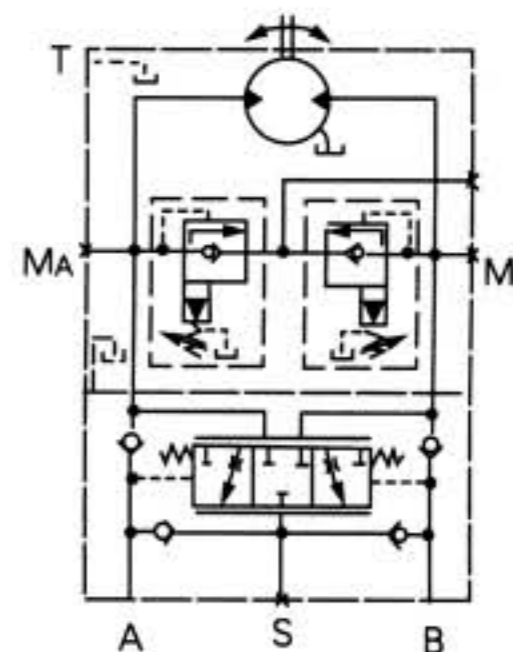
油口 connections
