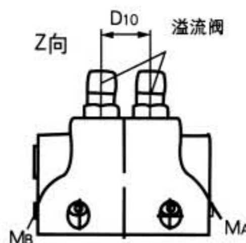
油口 connections
