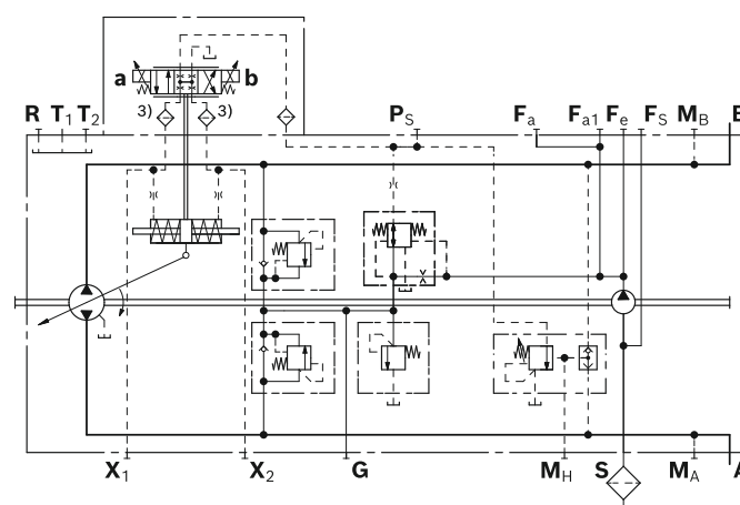
▼ Circuit diagram, version with DA control valve 2)
