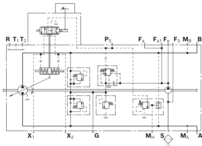
Correlation of direction of rotation, control and flow direction
