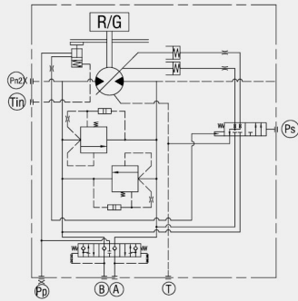
Hydraulic Circuit
