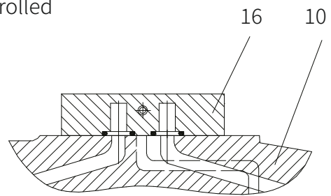
Model 4WRH...-7XJ/
