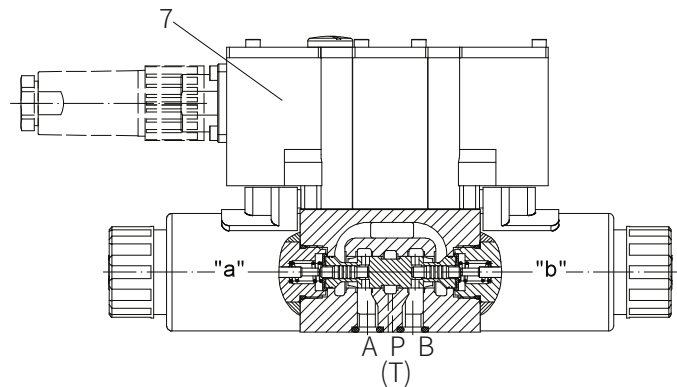
Model 3DREPE6...-2XT/
