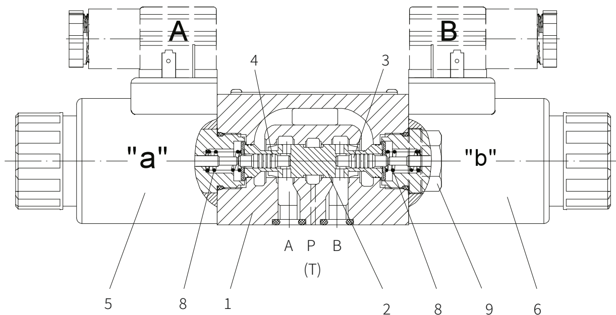
Model 3DREP6...-2XT/
