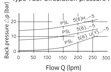
Type TSL: Circulation pressure P R(F)
