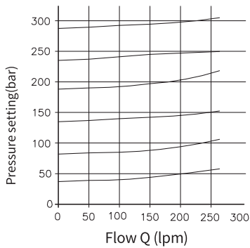
Pressure limiting valve Connection block
