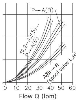
Directional spool valve P A(B), A(B) R
