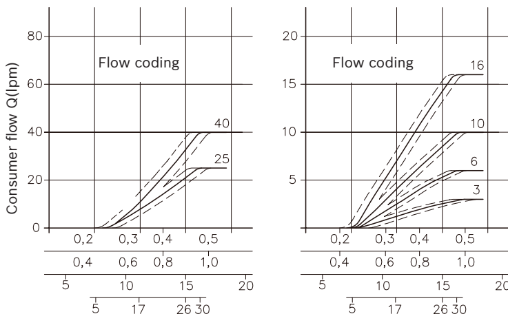
Control curve for consumer flow (Guide line, example for directional spool valve type SL 2-2../.. with inflow controller)
