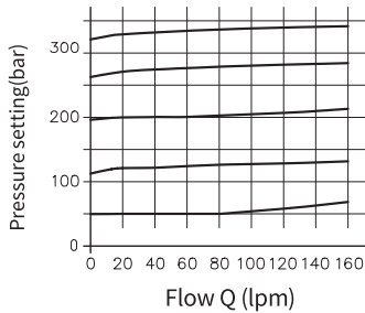
IS relief valve P-O curve
