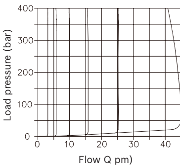
2-way inflow controllers
