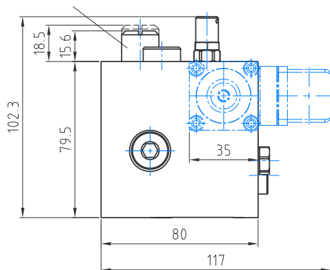
Three-way pressure reducing valve
