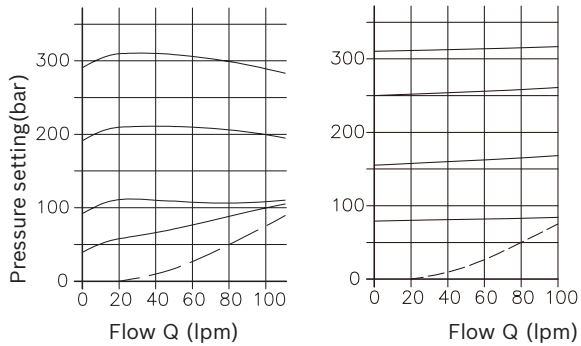
Pressure limiting valve in the connection block Type TSL 3../D../-2 TSV 3../D../-2
