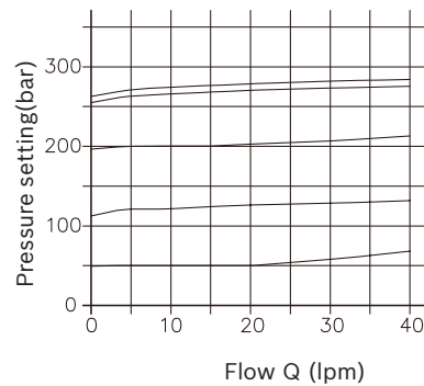
Prop. pressure limitation Coding FP(H) 1, (FP(H) 2, FPH) 3, table 17, sect. 3.2.1
