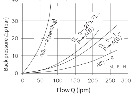
Back pressure(full elevation)
