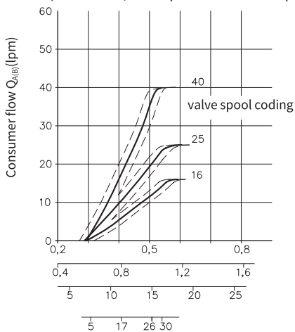
Input / consumer flow curve
