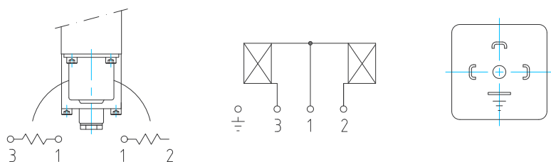
Pin definition of the twin solenoid
