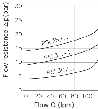
2-way inflow controllers
