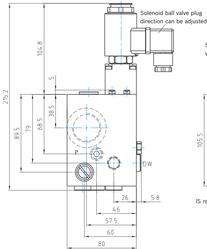
Three-way pressure reducing valve
