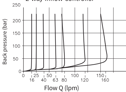
Input / consumer flow curve
